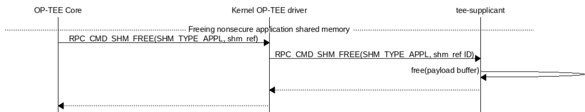
Fig. 10: Freeing previously allocated nonsecure shared memory
