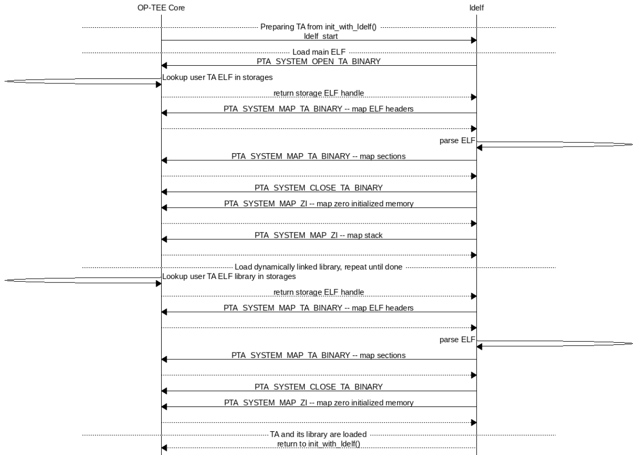
Fig. 11: Preparing TA for execution
