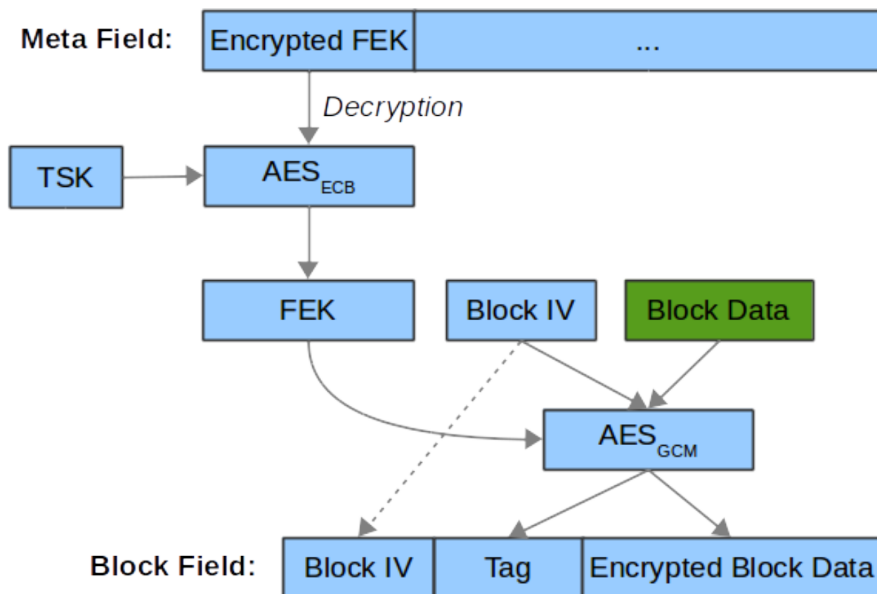
Fig. 8: Block data encryption
