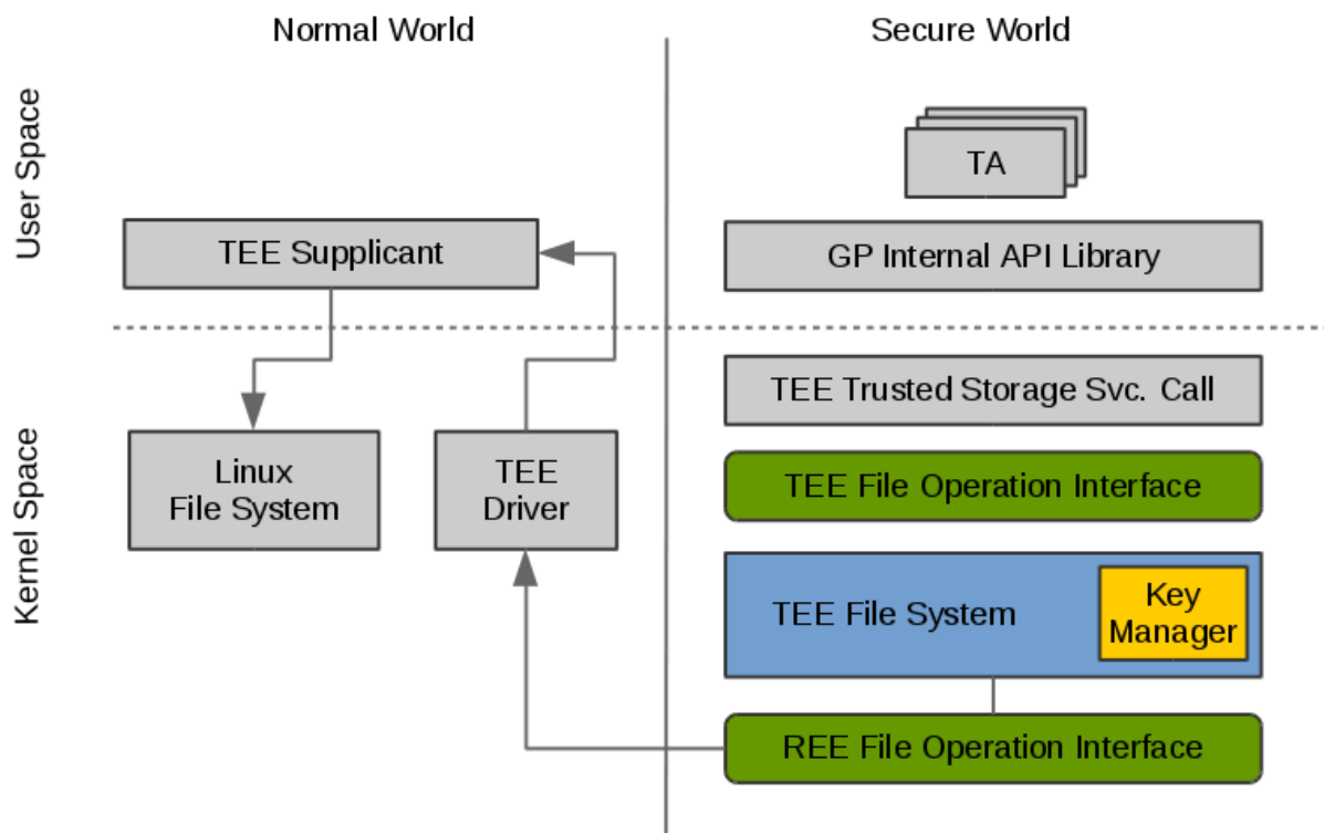
Fig. 6: Secure Storage System Architecture
