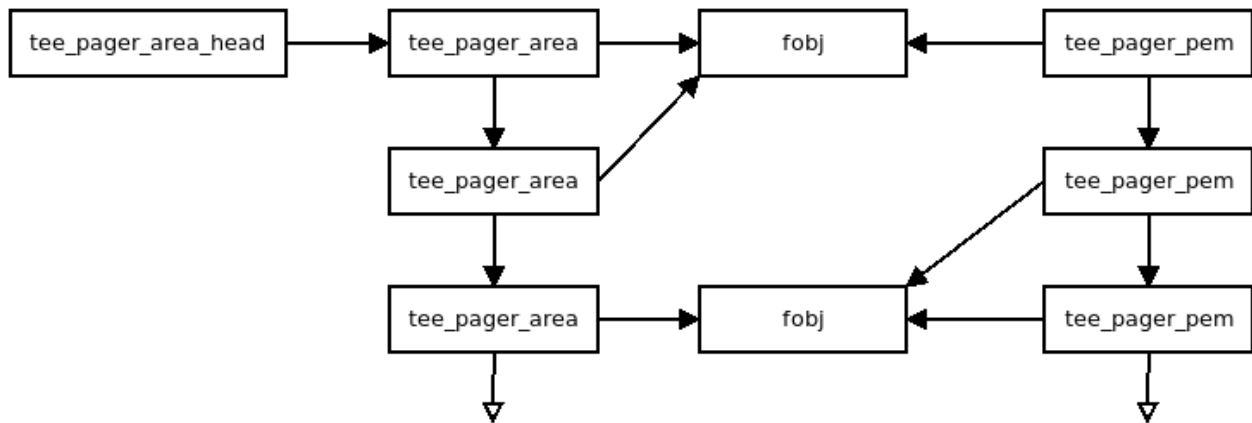
Fig. 5: How the main pager data structures relates to each other
