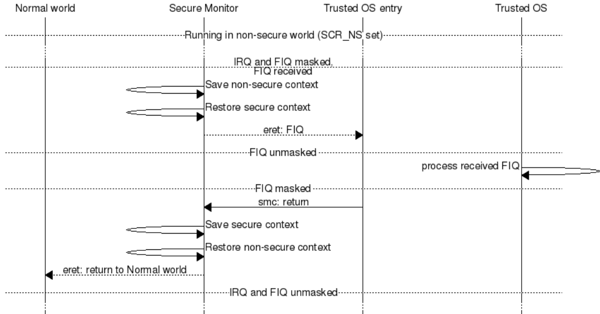
Fig. 3: FIQ received when SCR_NS is set
