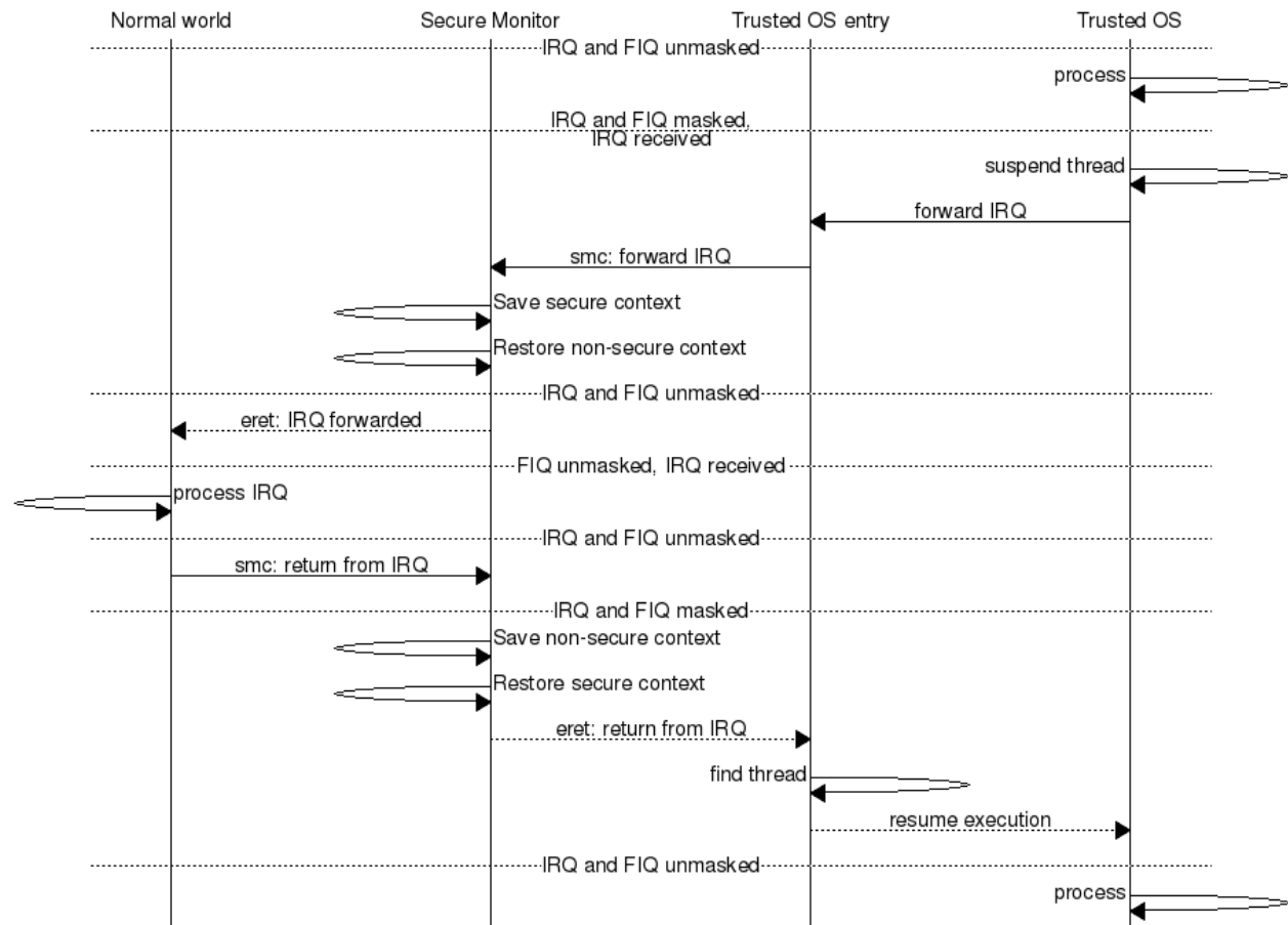
Fig. 2: IRQ received in secure world and forwarded to normal world
