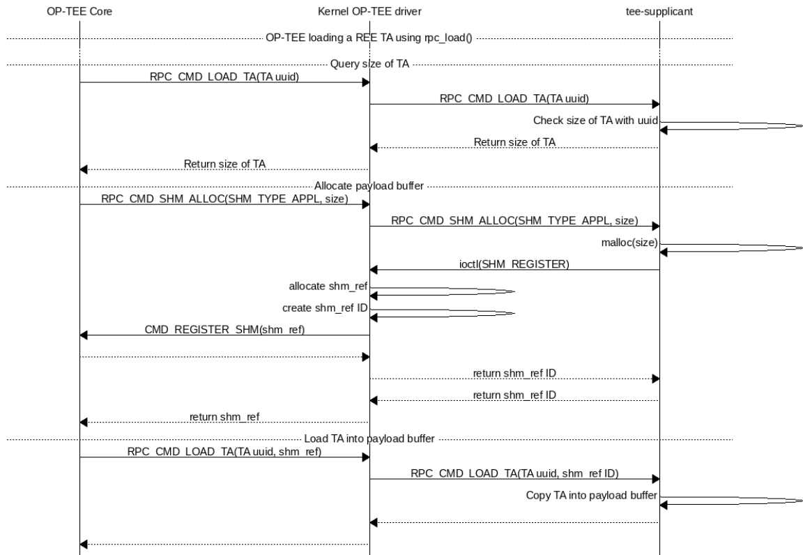
Fig. 9: Loading a REE TA into nonsecure shared memory
