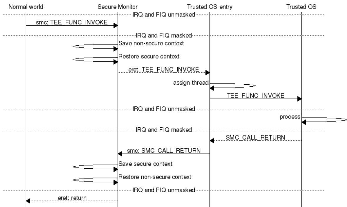
Fig. 1: SMC entry to secure world
