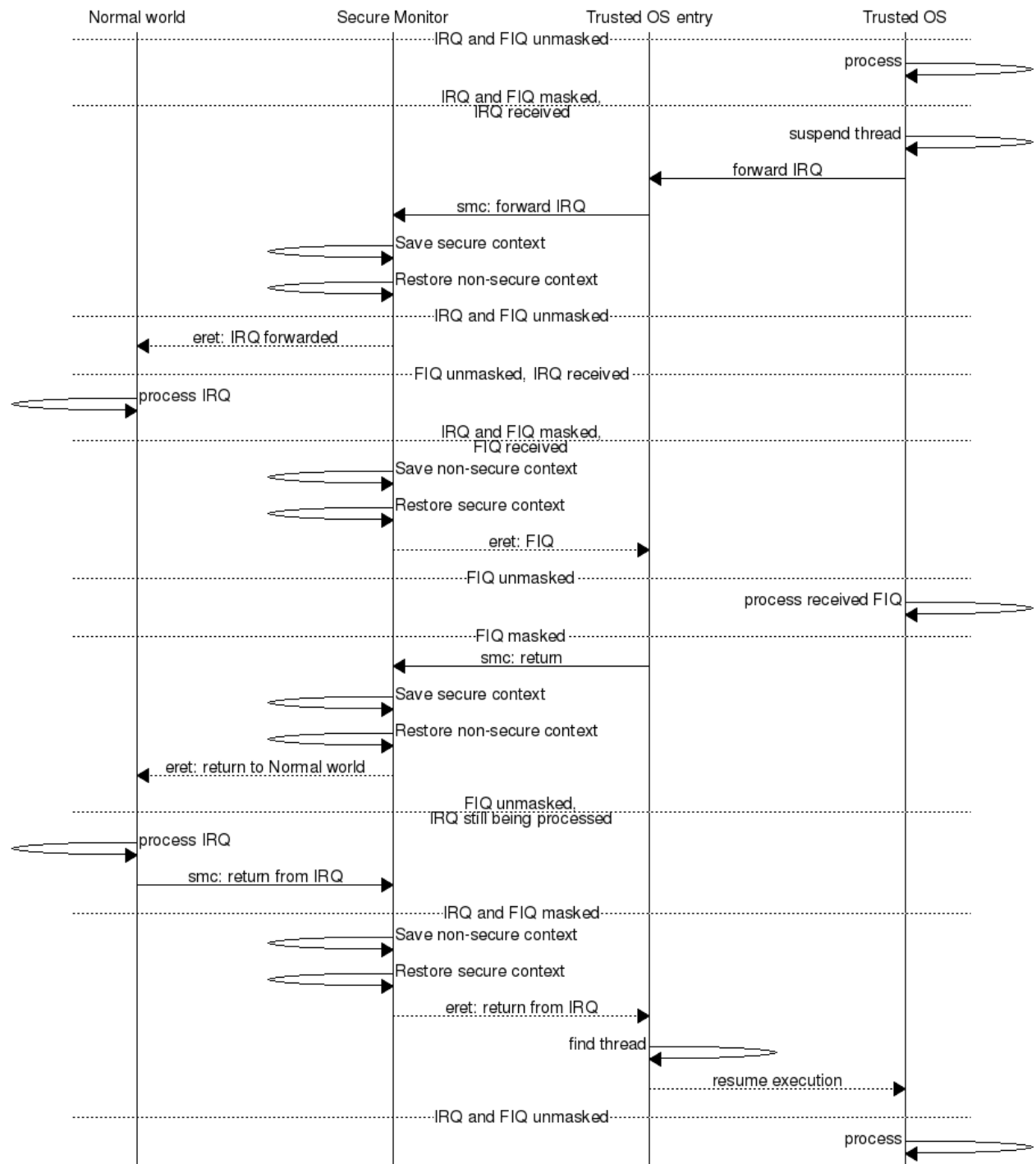
Fig. 4: FIQ received while processing an IRQ forwarded from secure world
