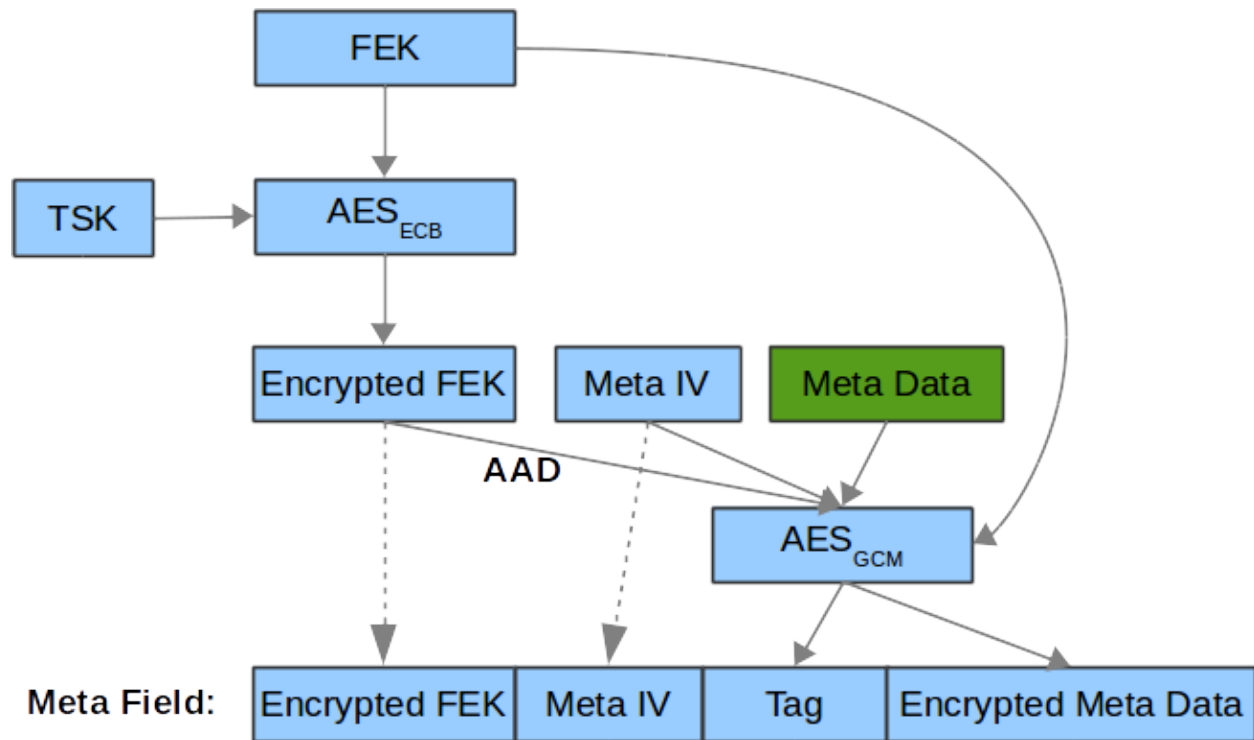
Fig. 7: Meta data encryption
